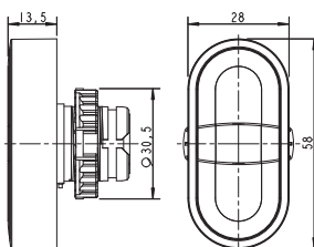
CSW-BD (illuminated center)
